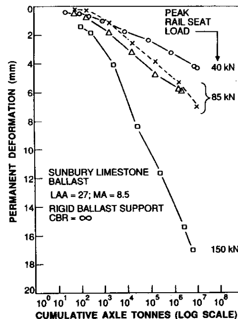
FIGURE 5 Accumulated permanent deformation (rigid ballast support).
