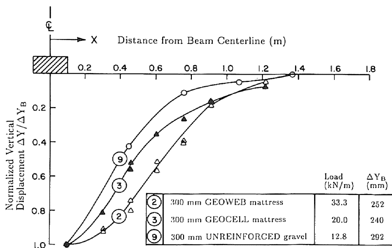
FIGURE 9 Deformation profiles at gravel base-peat interface for selected tests.
