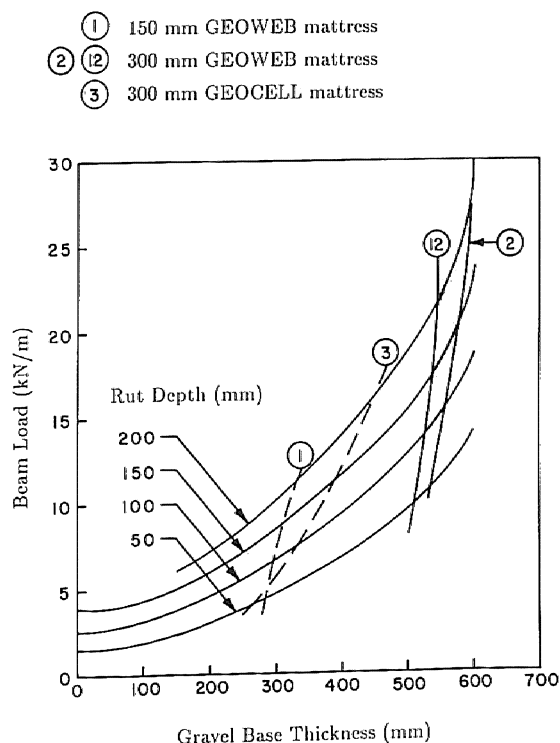
FIGURE 8 Equivalency chart for geocomposite mattress tests and unreinforced gravel bases (initial loading only).
