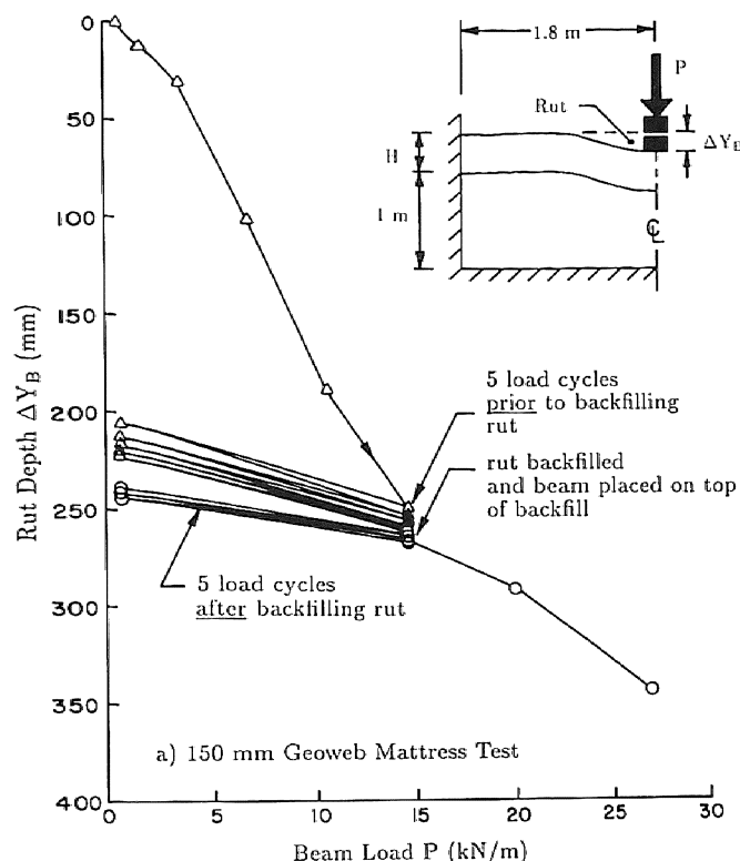
FIGURE 10 Load deformation for geocomposite mattress tests including backfilling and repeated static loading—150-mm geoweb mattress test.
