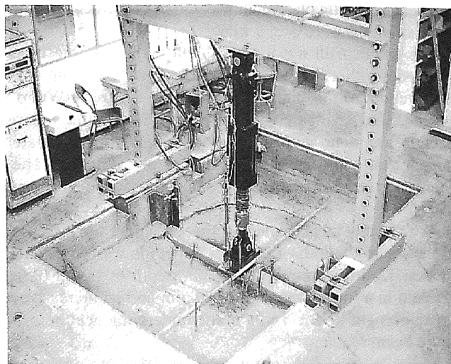
FIGURE 2 Overview of RMC test facility.
