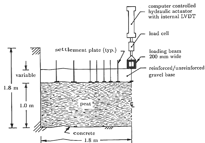
FIGURE 1 General test arrangement.
